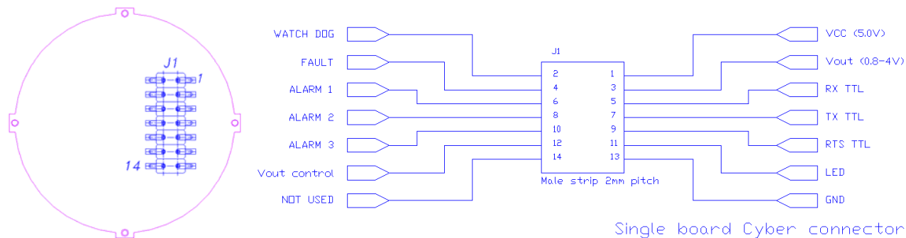
Figure 7.1 Single board Cyber connector and overview.
