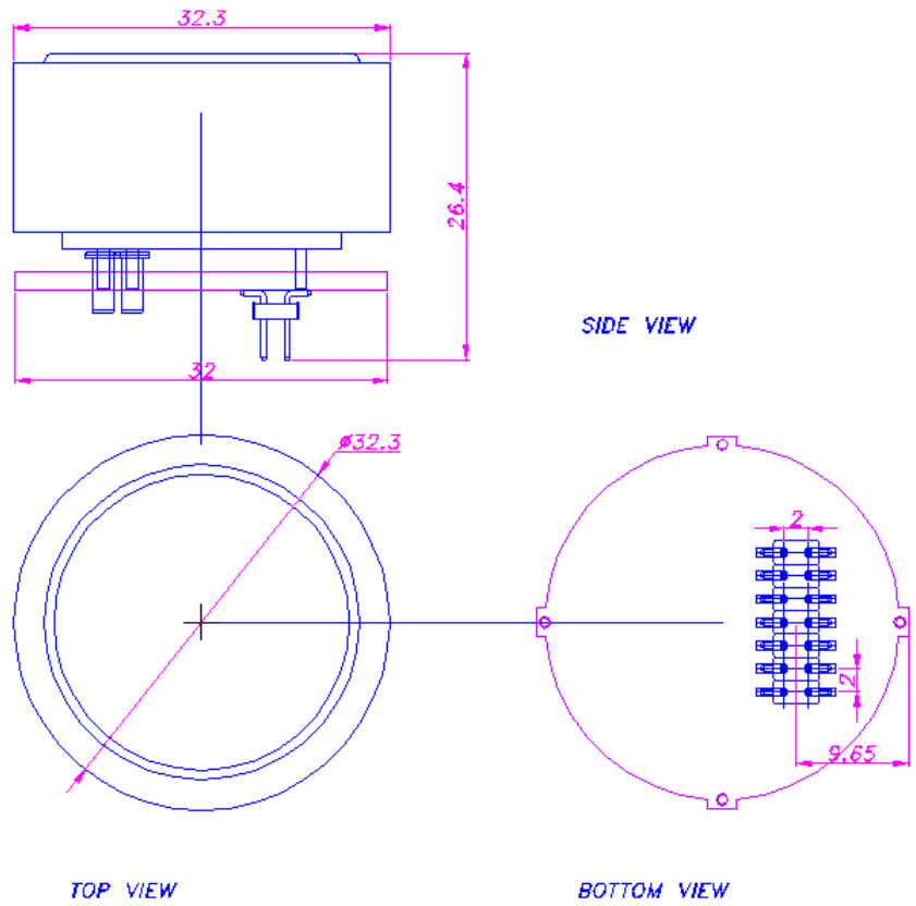
Figure 6.3 Electrochemical cell, 7 series type, for toxic gases detection;
