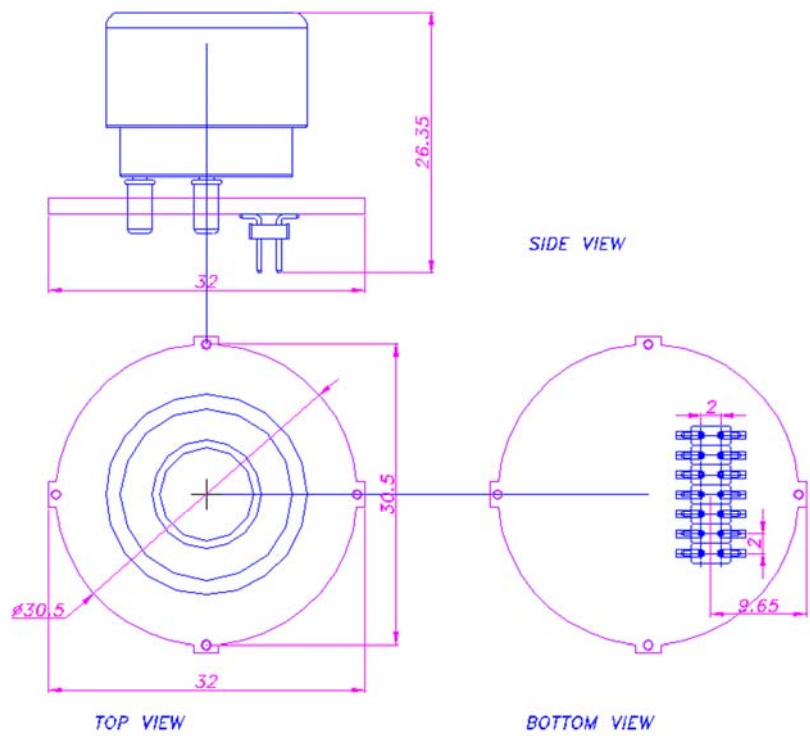
Figure 6.1 Single header industrial catalytic sensor for combustible gases;
