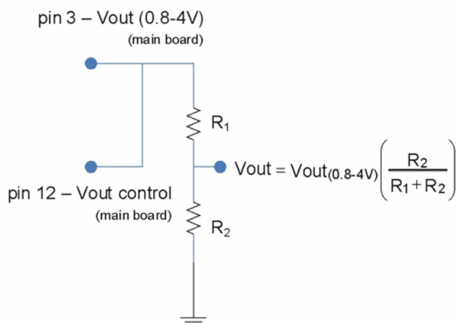
Figure 7.3 Vout value shifted down (in relation to 0.8—4V). The zero value at minimum 0.4V.
