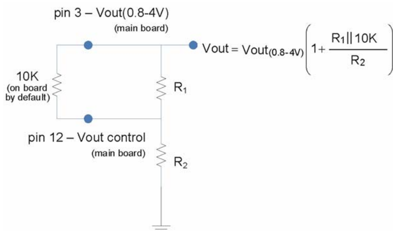
Figure 7.2 Vout value shifted up (in relation to 0.8—4V). The full scale value at maximum 5V.
