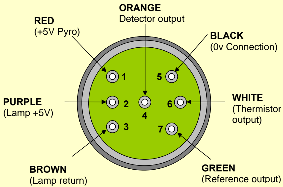
VIEW OF SENSOR SOCKETS. COLOURS REFER TO THE CONNECTING WIRES
