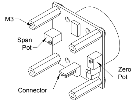
Figure 4. Mounting pillar configuration for attaching to the base of an enclosure.
