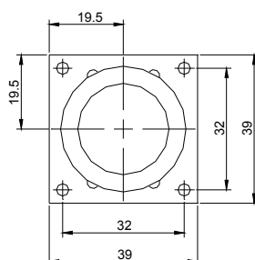
Figure 1. Outer mounting hole locations.
