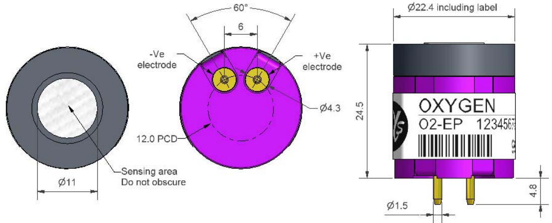
Figure 1 O2-EP Schematic Diagram
